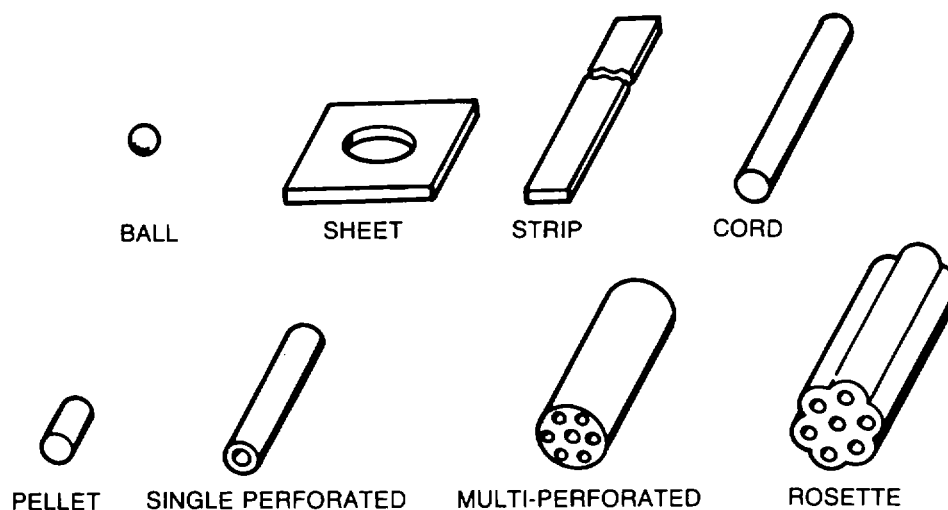
Figure 9-1. Typical shapes of propellant grains.
