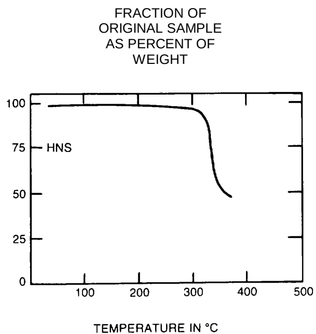
Figure 8-49. TGA curve for HNS.
