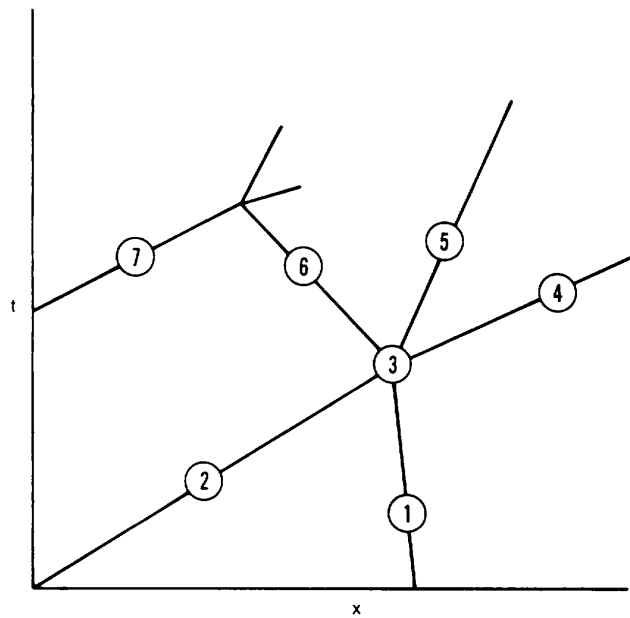
Figure 4-4. Shock properties in the x-t plane.
