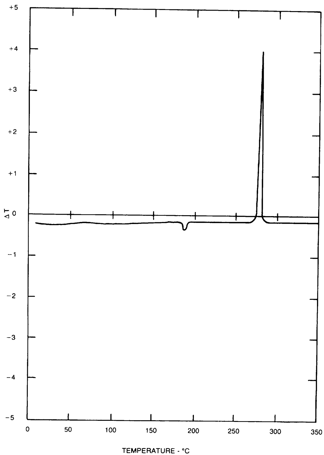
Figure 8-92. DTA curve for PBXN-5.
