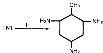
Figure 8-61. Reaction of TNT with hydrogen.
