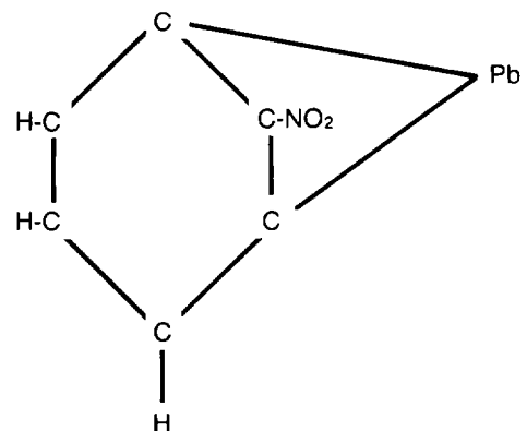
Figure 7-11. Structural formula for LMNR.
