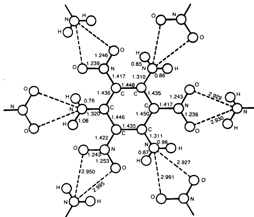
Figure 8-51. Configuration of the TATB molecule.
