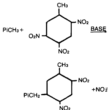
Figure 8-56. TNT and 2,4,5-TNT reaction.
