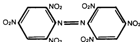
Figure 8-45. Structural formula for HNAB.
